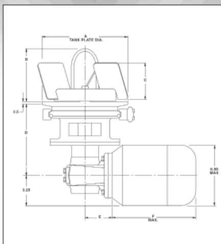
MagMixer MBI 205 (Dim. in inches)
