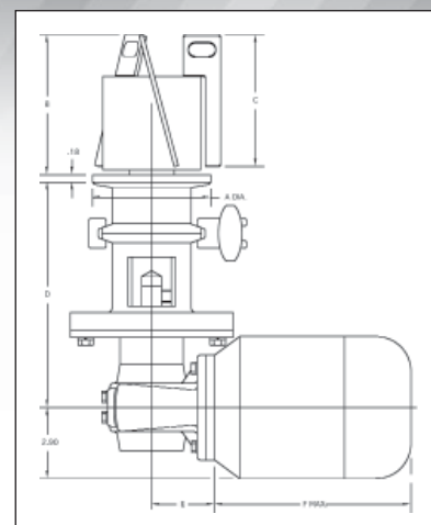
MagMixer MBI 205 (Dim. in inches)
